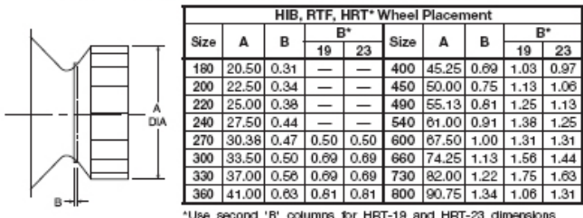
Figure 6. Wheel-Funnel Overlap
